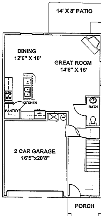
FIRST FLOOR 773 SQFT
