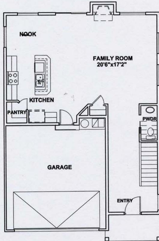
FIRST FLOOR 875 SQFT.
